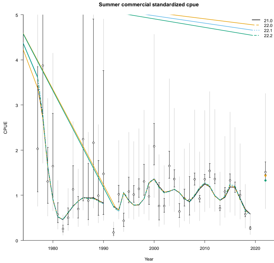
Figure 7. Observed (open circle) with 95% lognormal Confidence Intervals with additional variance (gray), and model estimated standardized CPUE.
