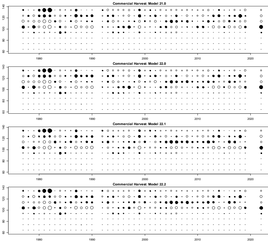
Figure 14. Bubble plots of predicted and observed length proportions. Black circles indicate model underestimates compared to observed, and white circles indicate model overestimates compared to observed. Size of circle indicates degree of deviance (larger circle = larger deviance). In ideal model fit case, distribution of sizes and colors of circles should be random (i.e., no systematic model misfits).
