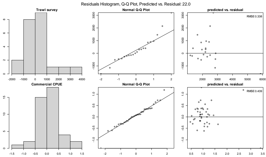
Figure 16. QQ Plot of Trawl survey and Commercial CPUE.
