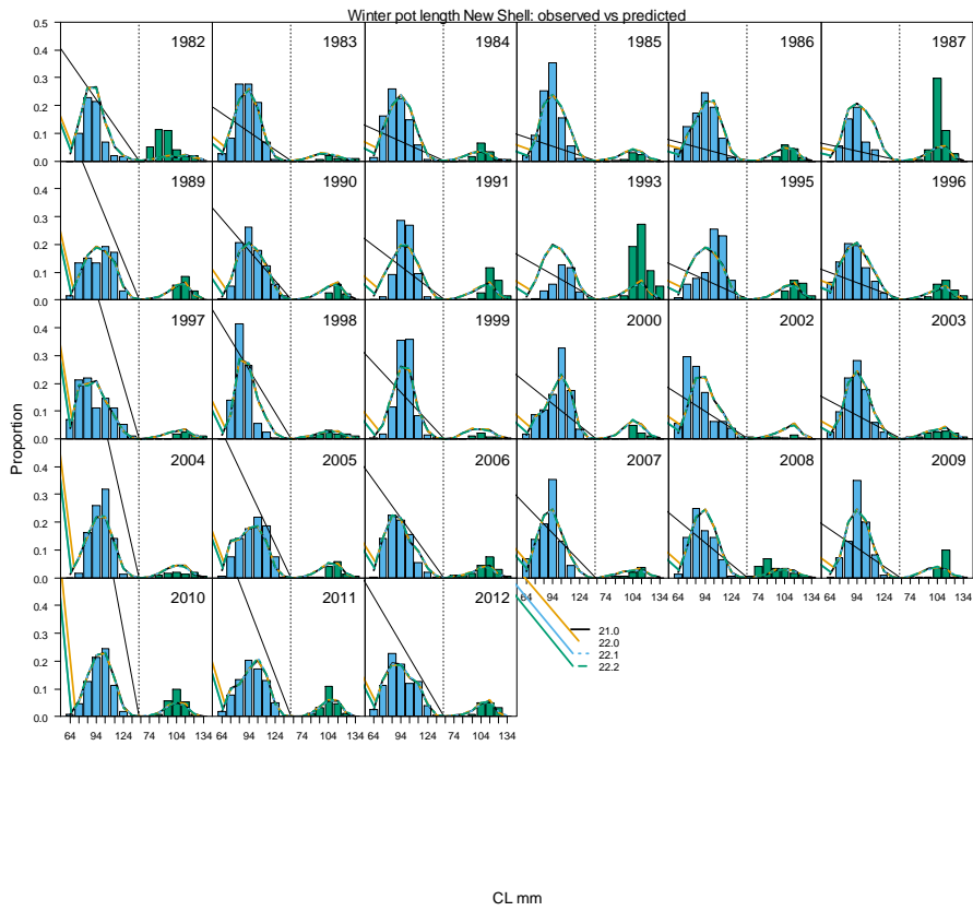
Figure 10. Predicted (line) vs. observed (bar New Shell: blue, Old Shell: green) length class proportions for winter pot survey 1982-2012.
