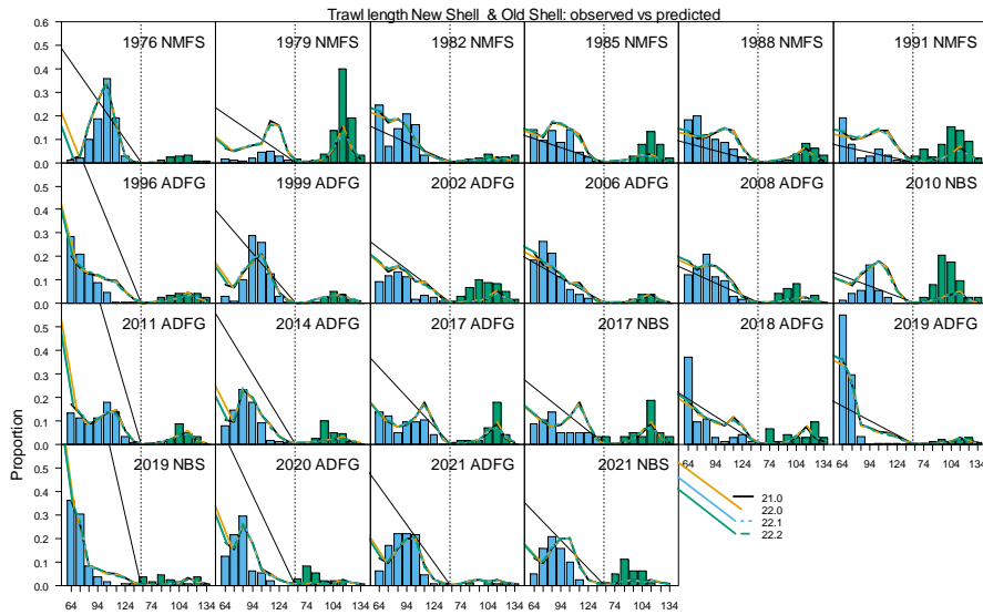
Figure 9. Predicted (line) vs. observed (bar New Shell: blue, Old Shell: green) length class proportions for trawl survey 1976-2021.
