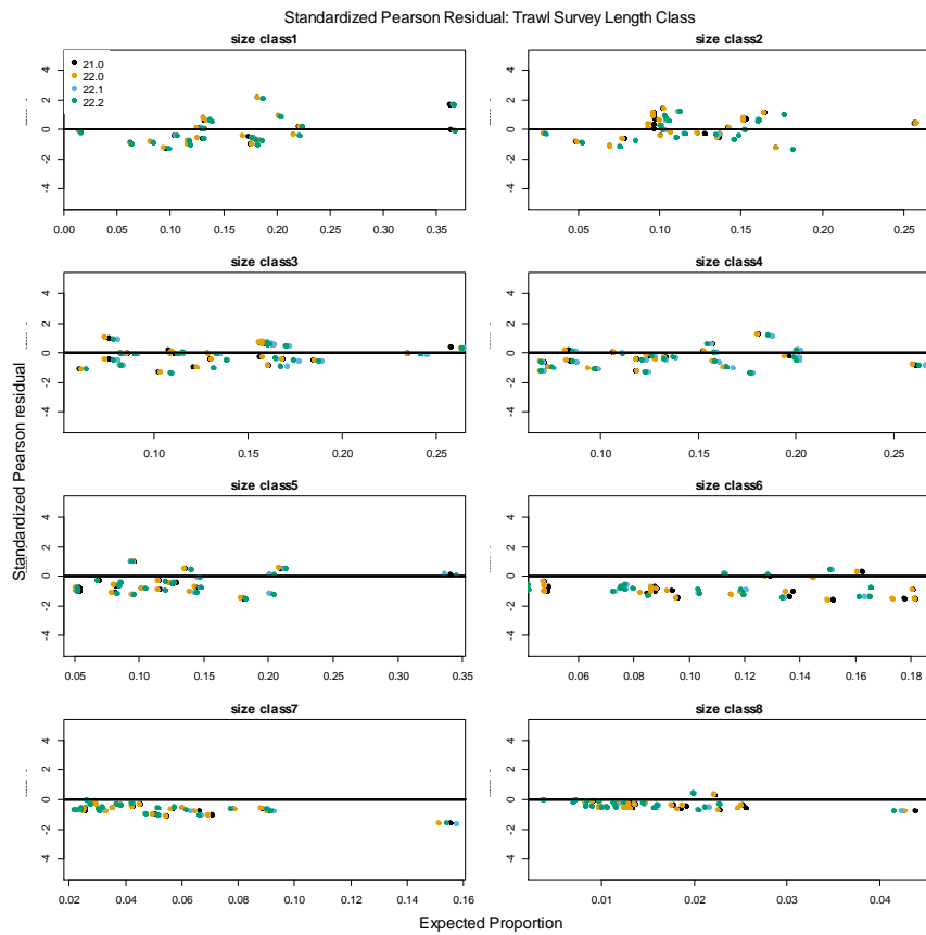
Figure 15. Standardized Pearson residual plots for trawl survey, summer commercial retained catch, winter pot survey, and observer for length size classes 1-8.
