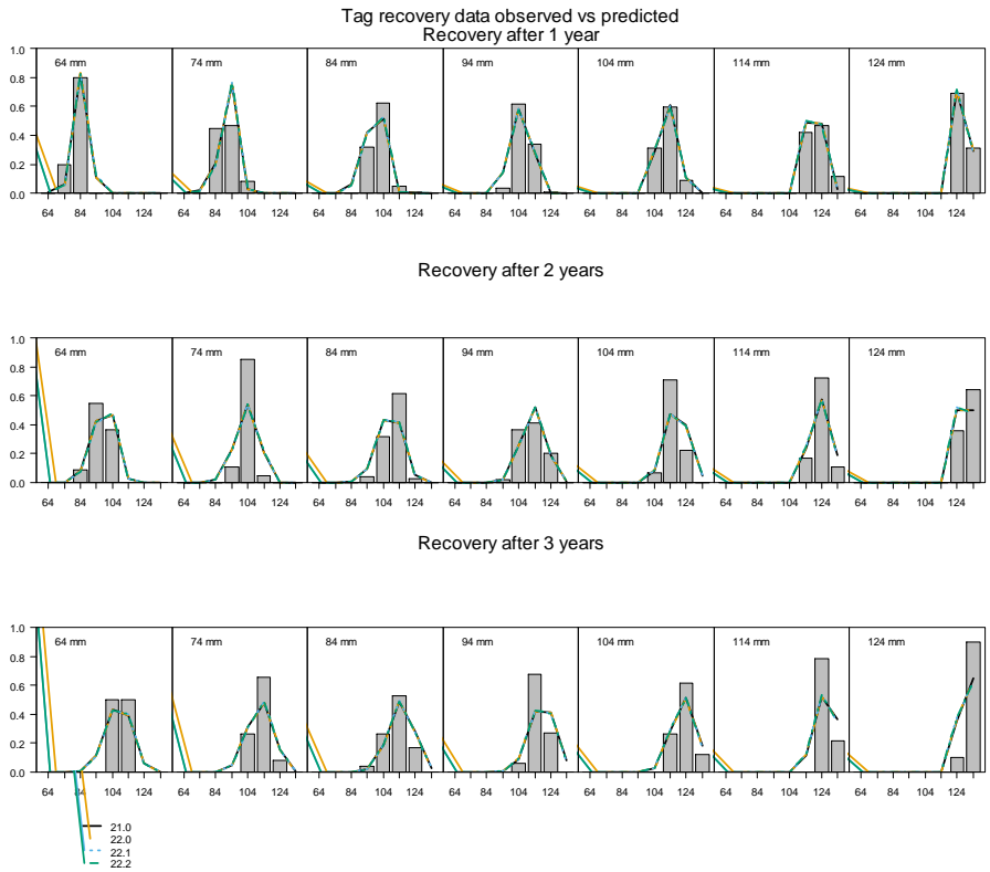
Figure 12. Predicted (line) vs. observed (bar) length class proportions for tag recovery data.
