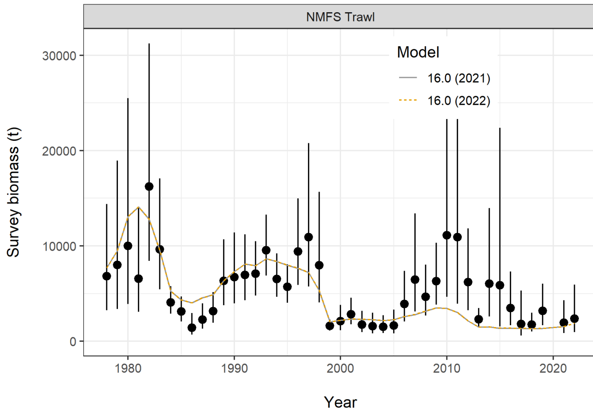
Figure 6: Fits to NMFS area-swept trawl estimates of total (> 90mm) male survey biomass for the base model only (16.0 ref for 2022 and 16.0 2021 accepted model). Error bars are plus and minus 2 standard deviations.
