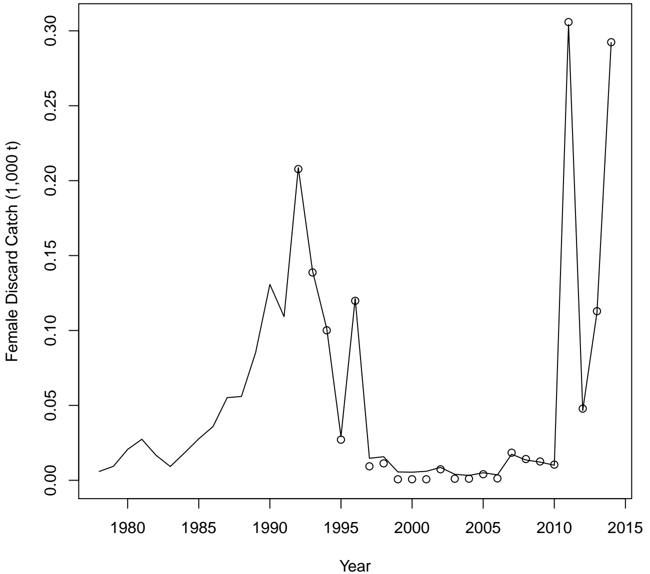
Figure 50. Model fit to female discard bycatch in the directed fishery from 1992/93 to 2014/15 and model estimates of discard from 1978 to 2014/15.
