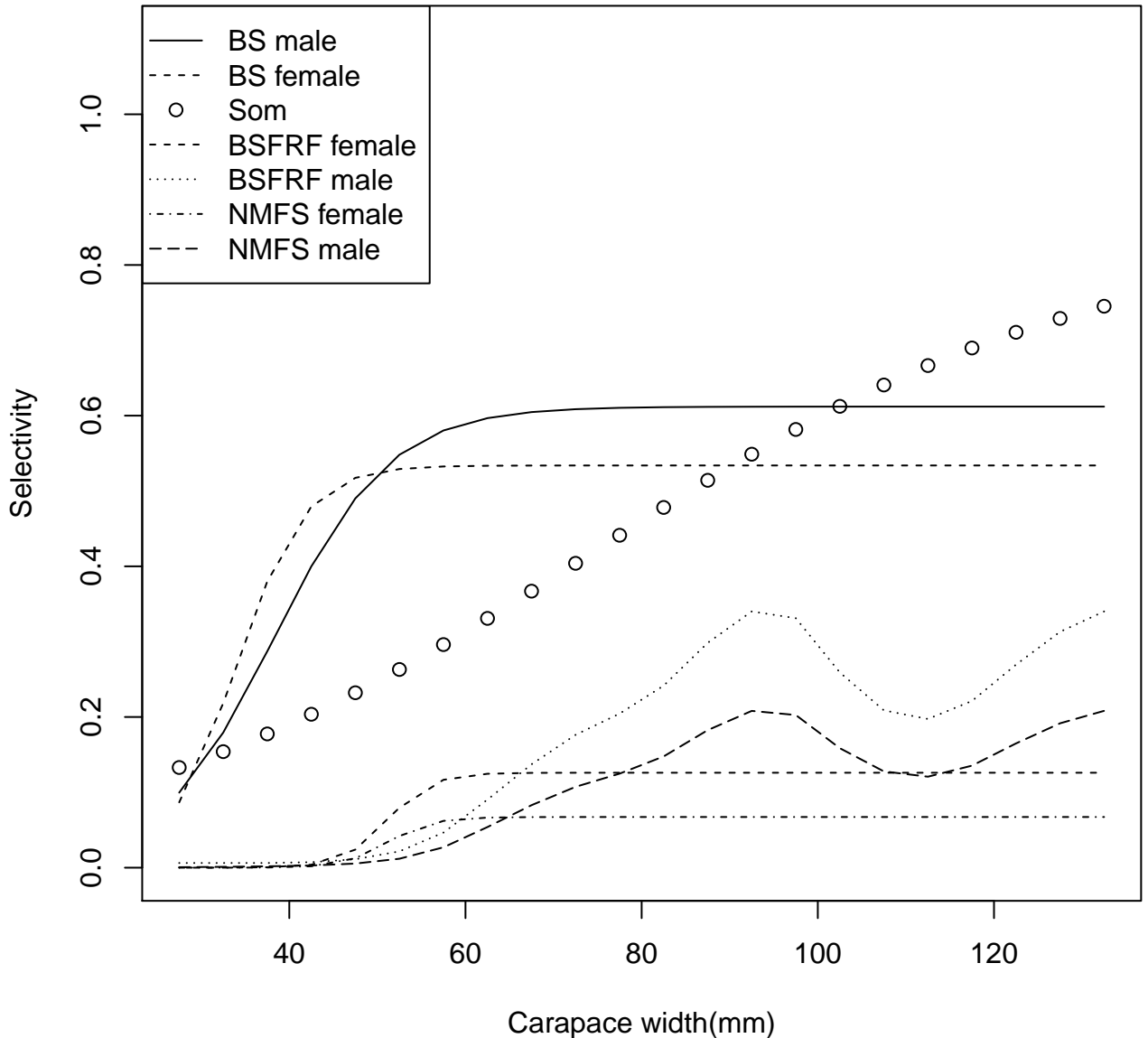
Figure 40. Survey selectivity curves entire Bering Sea survey for female (upper dashed line) and male snow crab (solid line) estimated by the model for 1989 to present. Survey selectivities estimated by Somerton(2010) from 2009 study area data are the circles. Lower lines are survey selectivities in the study area for BSFRF male and female crab and NMFS male and female crab.
