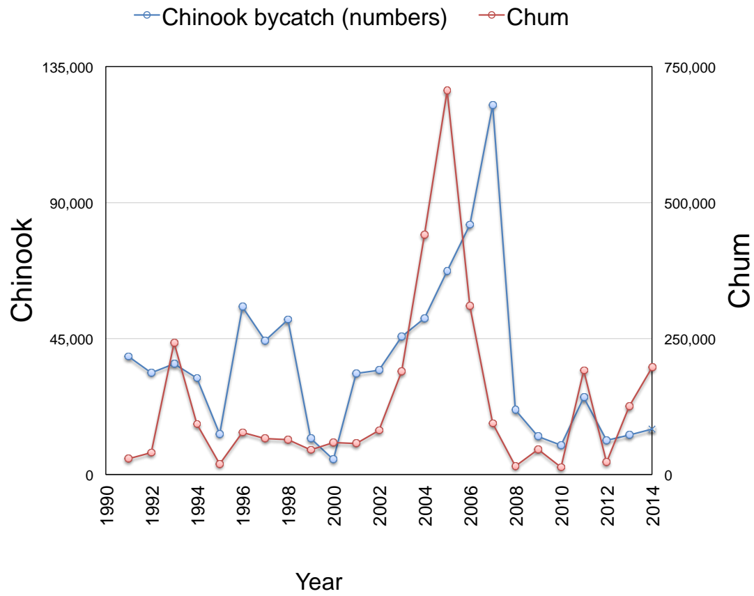
Time series of Chinook and chum salmon bycatch in the pollock fishery, 1991-2014.
